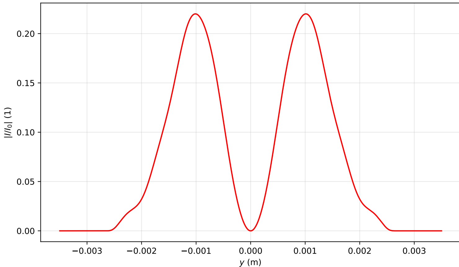
Intensity profile I(x=0, y, z=3.662)/I_0 , P_{in}=1.0P_{cr} , artificial time
